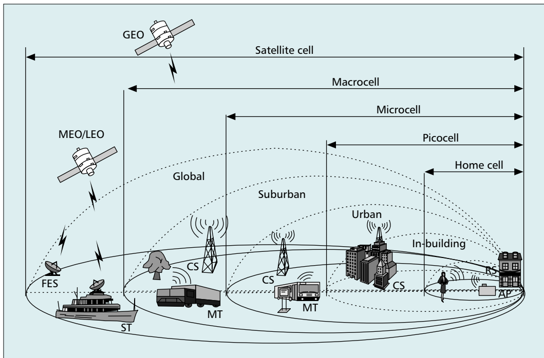
■ Figure 4. Cell hierarchy of a next-generation network.
