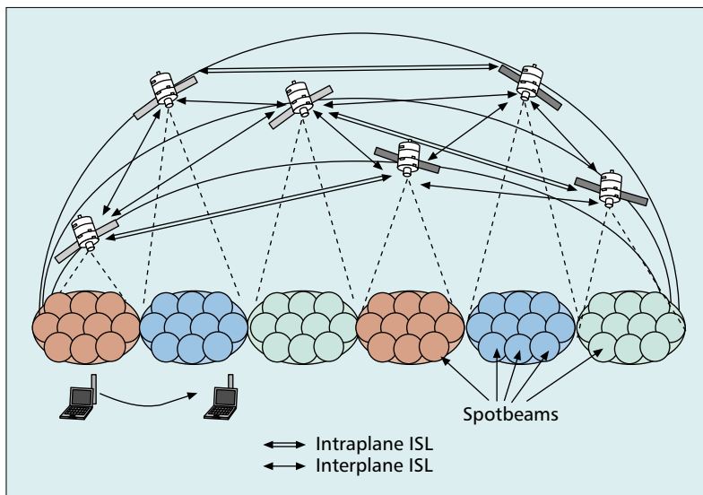
■ Figure 3. Reference architecture of a LEO satellite network.
