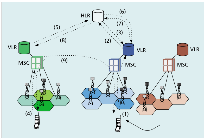
■ Figure 2. Reference architecture of a 2G network.
