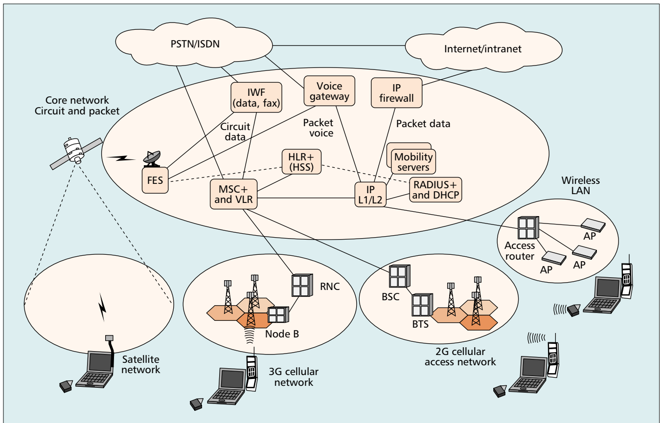
■ Figure 5. An all-IP wireless/mobile network.
