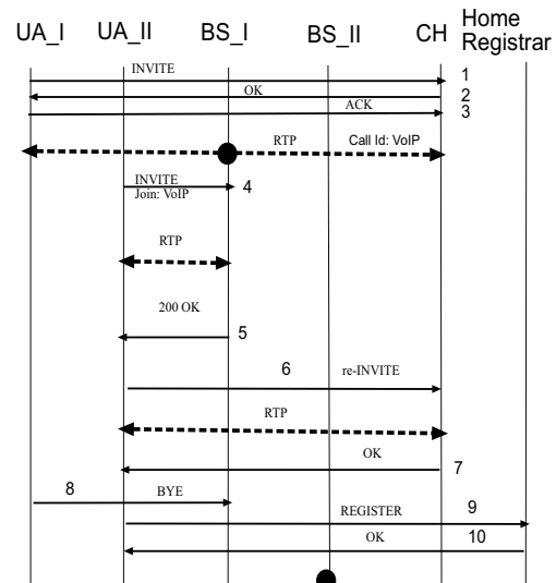
Figure 8. Message Diagram
