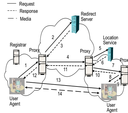
Figure 1. SIP architecture
