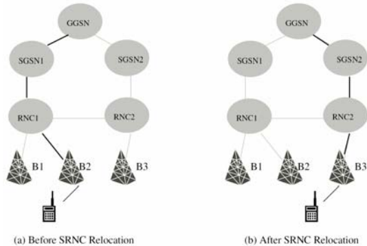
Fig. 2.9 Combined Hard Handoff with SRNS Relocation
