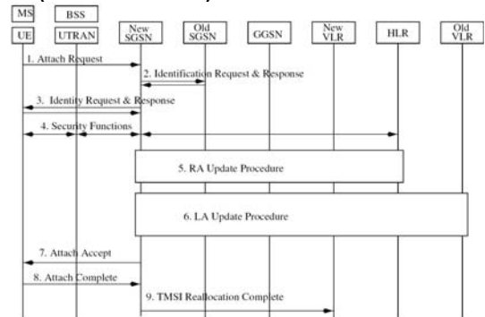
Fig. 2.6 Combined PS/CS (GPRS/IMSI) Attach Procedure
