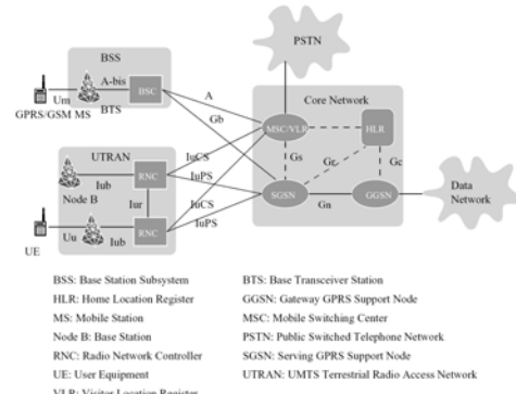
Fig. 2.1 GSM/GPRS/UMTS Network Architectures
