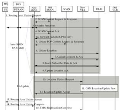
Fig. 2.7 Combined RA/LA Update
