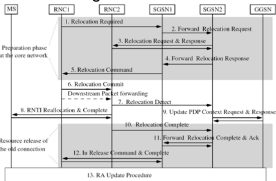
Fig. 2.11 SRNC Relocation Message Flow for PS
