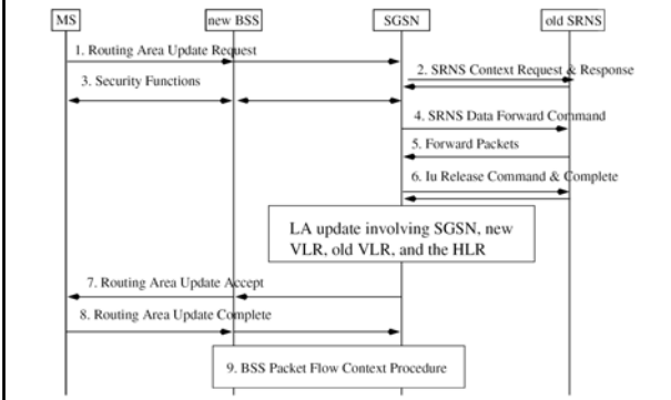
Fig. 2.12 Intra-SGSN Change from UMTS to GPRS
