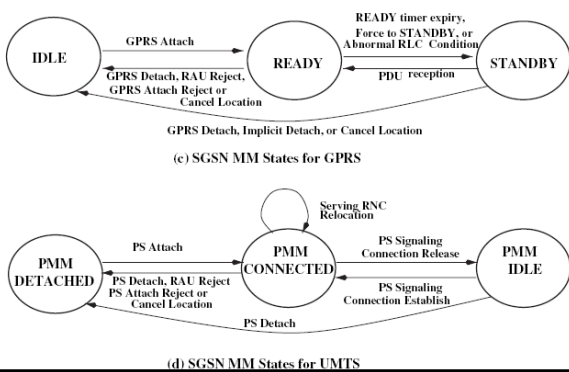
Fig. 2.5 SGSN MM State Diagrams
