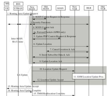
Fig. 2.7 Combined RA/LA Update
