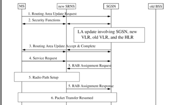
Fig. 2.13 Intra-SGSN Change from GPRS to UMTS
