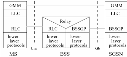
(b) Control Plane for GPRS Mobility Management
