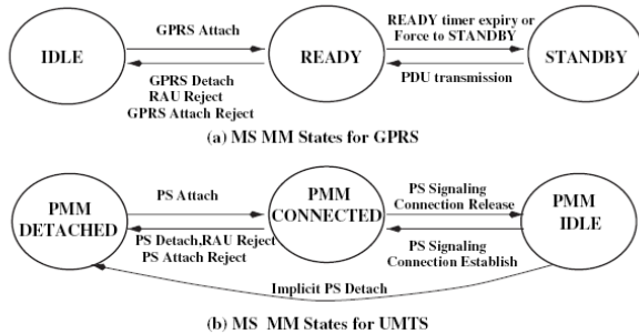
Fig. 2.5 MS MM State Diagrams
