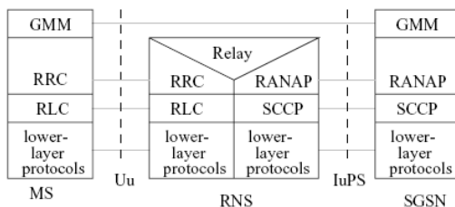
(a) Control Plane for UMTS Mobility Management
