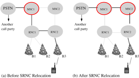
Fig. 2.10 CS SRNC Relocation
