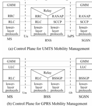
Fig. 2.2 Control Planes for UMTS and GPRS
