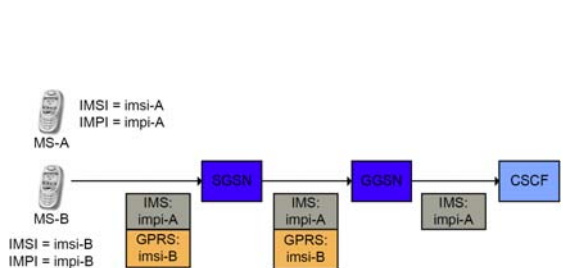
Fig.16.9 Illegal IMS Registration
