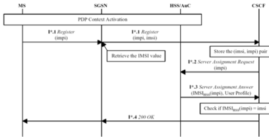
Fig.16.10 IMS Registration
