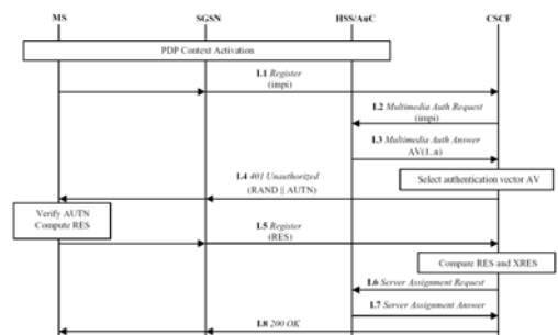
Fig.16.8 Message Flow for the 3GPP IMS Authentication
