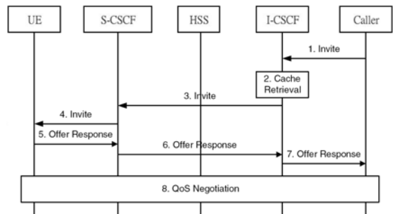
Fig.16.5 Incoming Call Setup with Cache Retrieval for C Schemes
