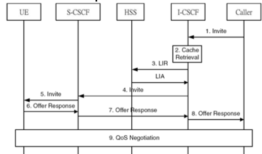
Fig.16.7 First Incoming Call Setup after I-CSCF-Failure: Cache Miss for Checkpoint Scheme 2
