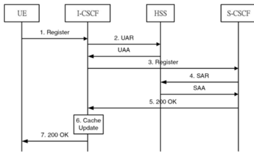
Fig.16.4 Registration with Cache Update for the C Schemes
