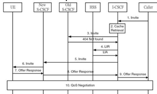
Fig.16.6 First Incoming Call Setup after I-CSCF-Failure: Cache Miss for the Checkpoint Scheme 1
