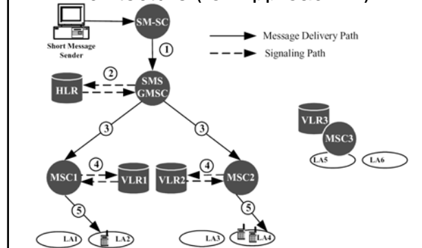
Fig. 11.4 Short Message Multicast Architecture (for Approach III)
