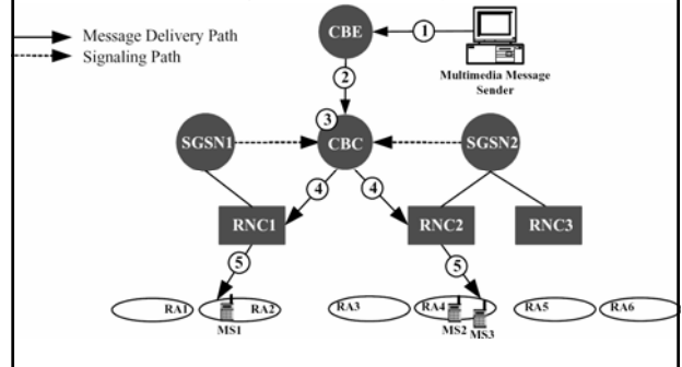
Fig. 11.7 UMTS Multimedia Message Multicast Architecture (PS Domain)
