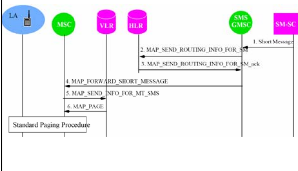
Fig. 11.6 The Multicast Procedure in Approach III
