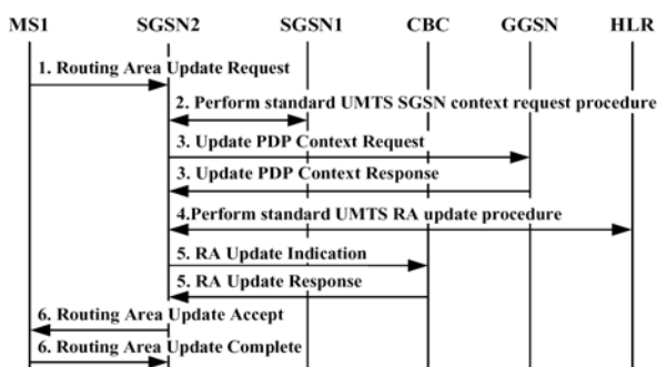
Fig. 11.10 Location Update Procedure for a Multicast Member
