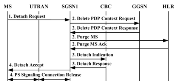
Fig. 11.9 Detach Procedure for a Multicast Member
