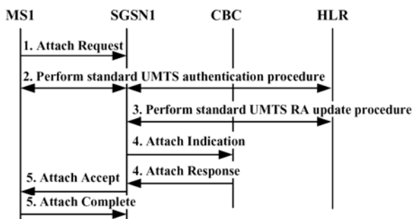
Fig. 11.8 Attach Procedure for a Multicast Member
