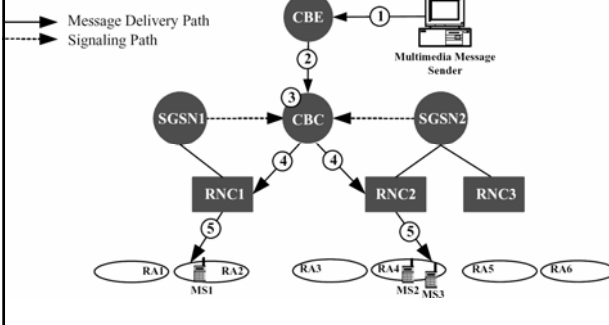
Fig. 11.7 UMTS Multimedia Message Multicast Architecture (PS Domain)
