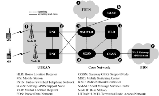
Fig. 11.3 UMTS Network Architecture (with SM-SC and WAP Gateway)
