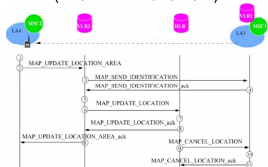
Fig. 11.5 Registration for a Multicast Member in Approach III (Inter-VLR Movement)
