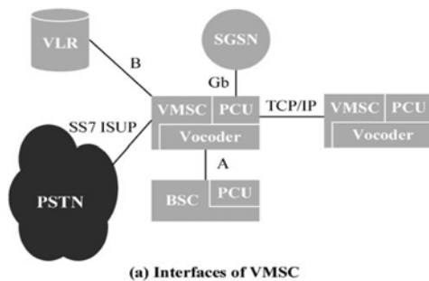
Fig. 10.12 The VMSC Interfaces and the VGPRS Network Architecture
