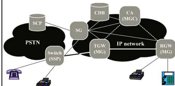
Fig. 10.1 The MGCP-Based VoIP Architecture
