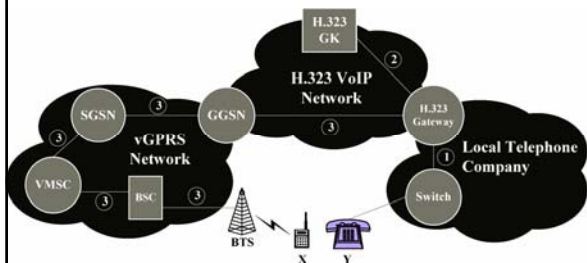
Fig. 10.20 Tromboning Elimination in vGPRS
