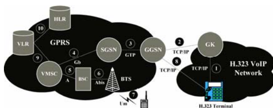
Fig. 10.13 Connection between an H.323 Terminal and a GSM MS
