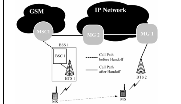
Fig. 10.10 Call Path for Inter-System Handoff
