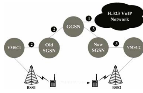
Fig. 10.17 The Routing Path before and after Inter-System Handoff
