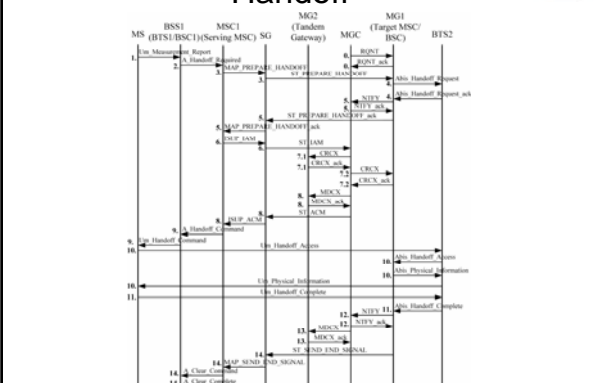
Fig. 10.11 Message Flow for GSM-IP Handoff
