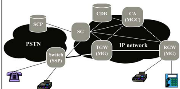
Fig. 10.1 The MGCP-Based VoIP Architecture
