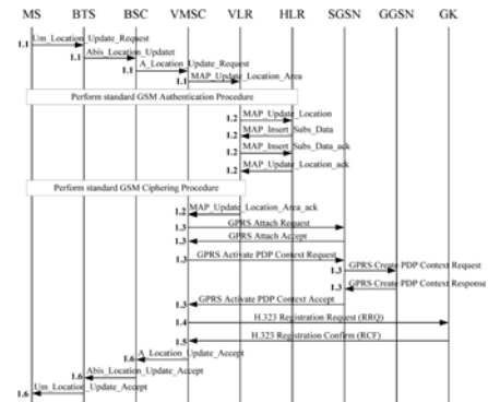
Fig. 10.14 Message Flow for vGPRS Registration
