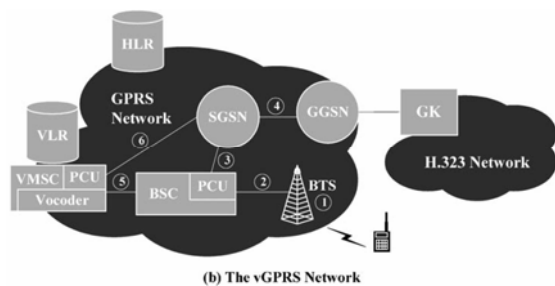
Fig. 10.12 The VMSC Interfaces and the VGPRS Network Architecture
