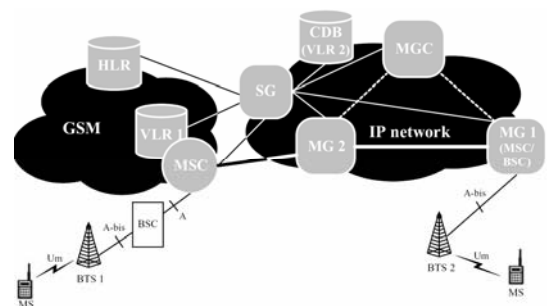
Fig. 10.4 The GSM-IP Architecture
