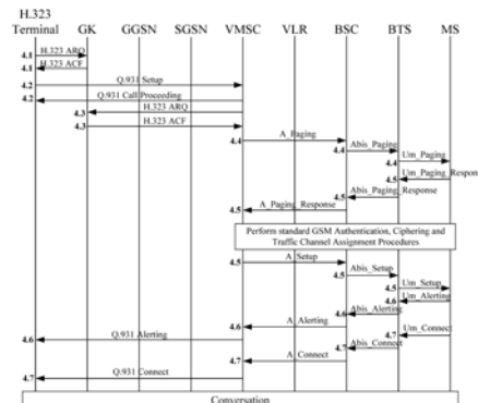
Fig. 10.16 Message Flow for MS Call Termination
