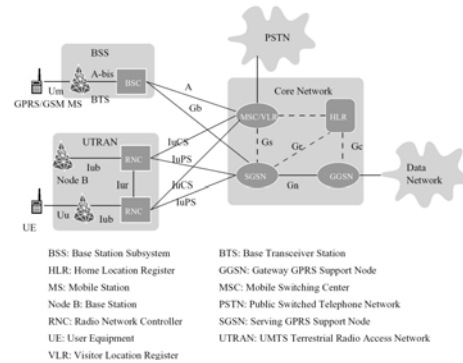
Fig. 2.1 GSM/GPRS/UMTS Network Architectures
