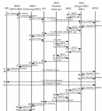
Fig. 10.11 Message Flow for GSM-IP Handoff
