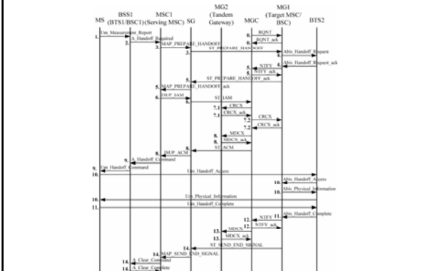
Fig. 10.11 Message Flow for GSM-IP Handoff
