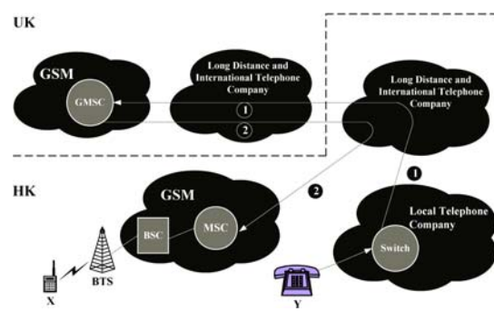
Fig. 10.19 Tromboning Phenomenon in GSM
