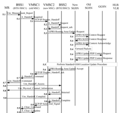
Fig. 10.18 The Message Flow for Inter-System Handoff
