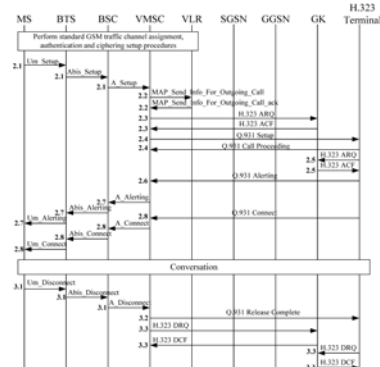
Fig. 10.15 The Message Flows for MS Call Origination and Call Release
