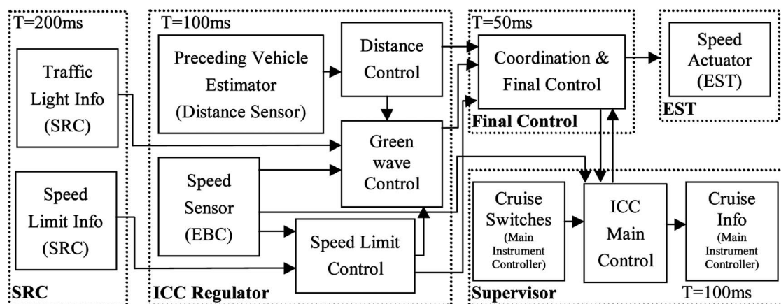
Fig. 18. AICC call-graph.
