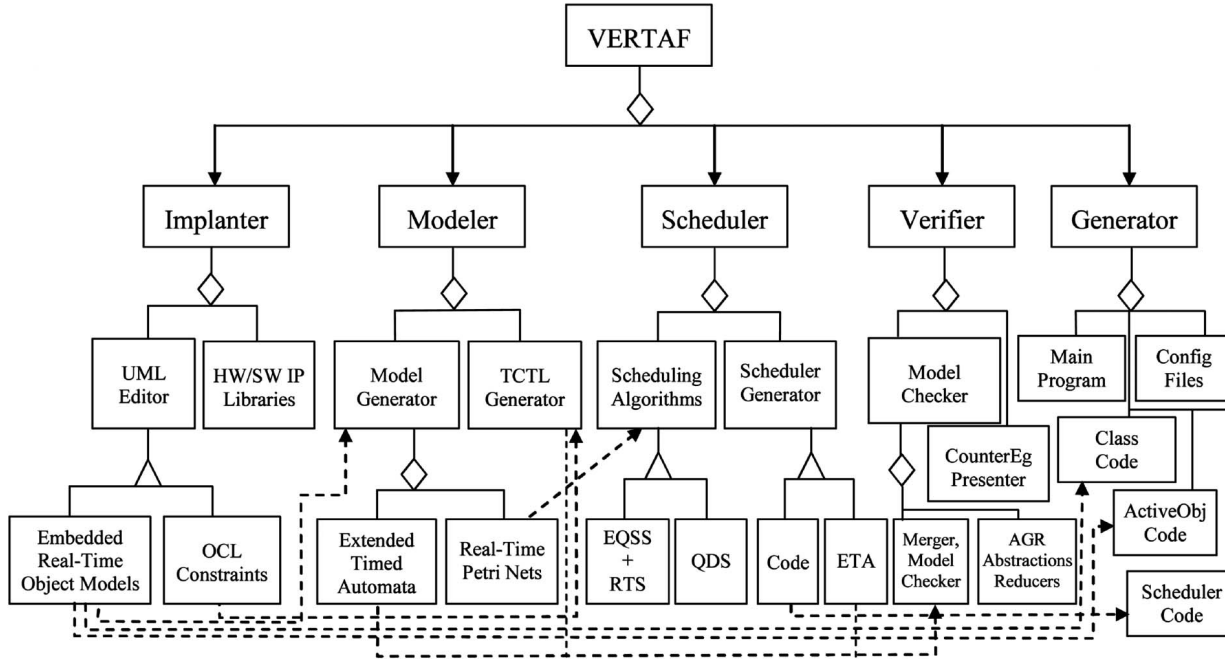
Fig. 14. Component view of VERTAF.
