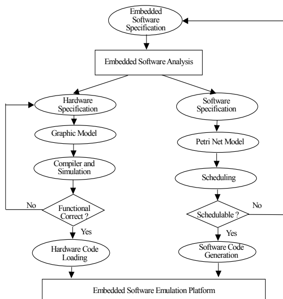
Figure 1 Embedded Software Synthesis and Prototyping Methodology
