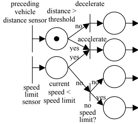
Figure 2 Automatic Cruise Controller CCPN Model
