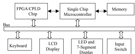
Figure 3 Hardware-Software Prototype Platform Architecture
