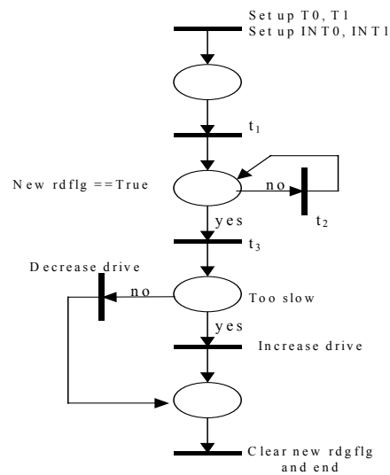
Figure 6 Motor Control Speed System CCPN Model
