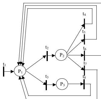
Figure 4 Petri Net Model of Display System
