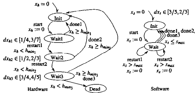
Figure 4: Hardware Concurrency
