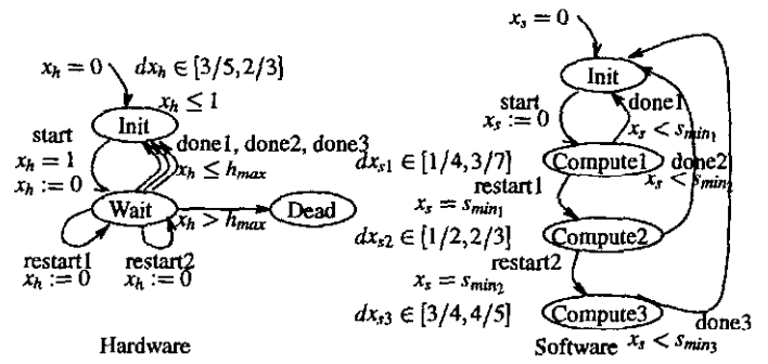
Figure 3: Software Concurrency
