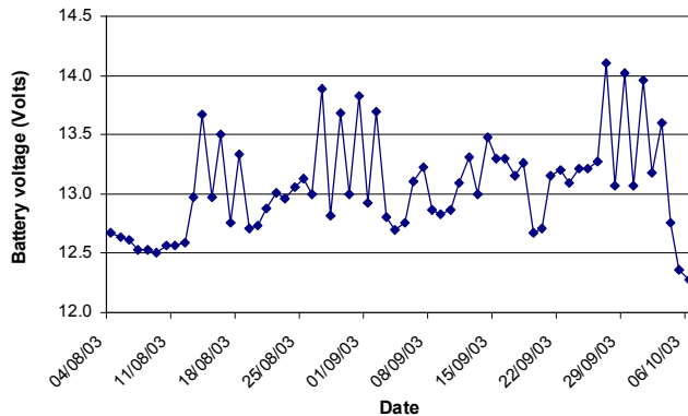
Figure 8. Base Station battery Voltage
