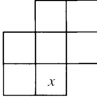
Fig. 2. The support region of the 3 \times 3 NSHP model, where x is the current predicted pixel.
